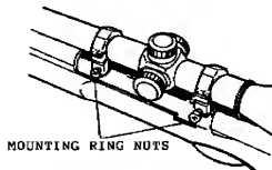
Figure 2-8. Ring nuts.
